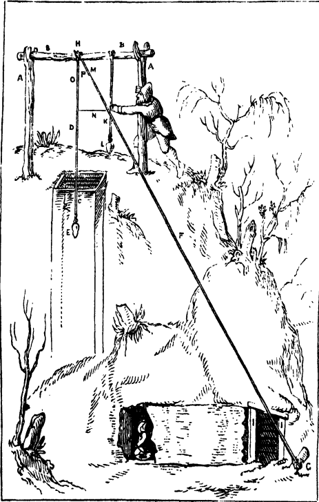
Fig. 147. The Adit Level. A, A . Two uprights or yokes supporting a bearer B B . C . The well, pit, or shaft. D . First cord. E . Weight of the first cord. F . The second cord, fixed to the earth at G . H, H . Head or ends of cords. I, I . The mouth or entrance of the adit or tunnel. K . The third cord, with weight attached, L, M . The first measure; N, N , the second; O , the third, forming the triangle P . (Agricola.)
